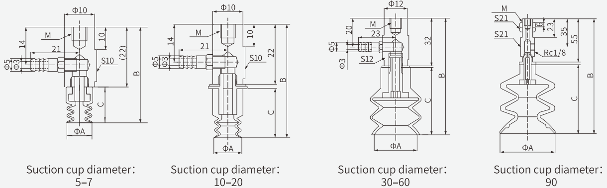
Lateral direction connection-Pagoda fitting
